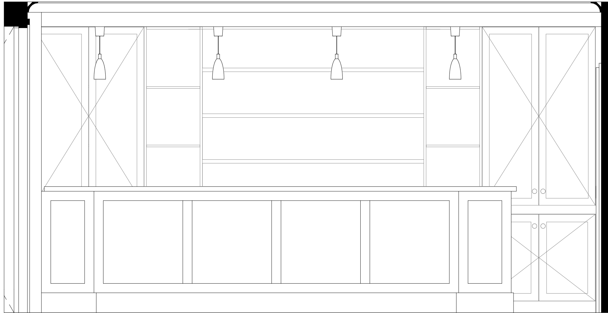
A - SECTION, 1:20
