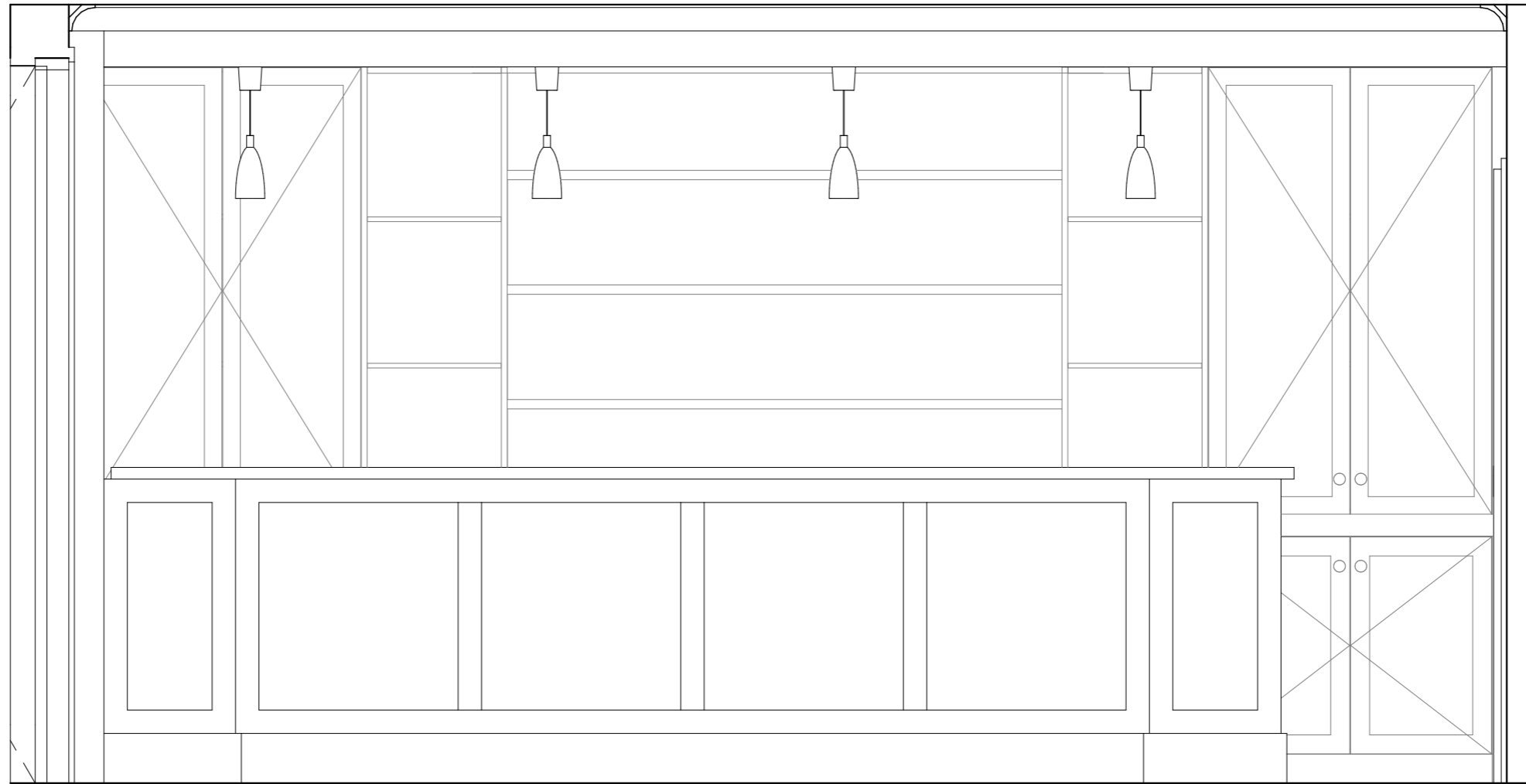
A - SECTION, 1:20
